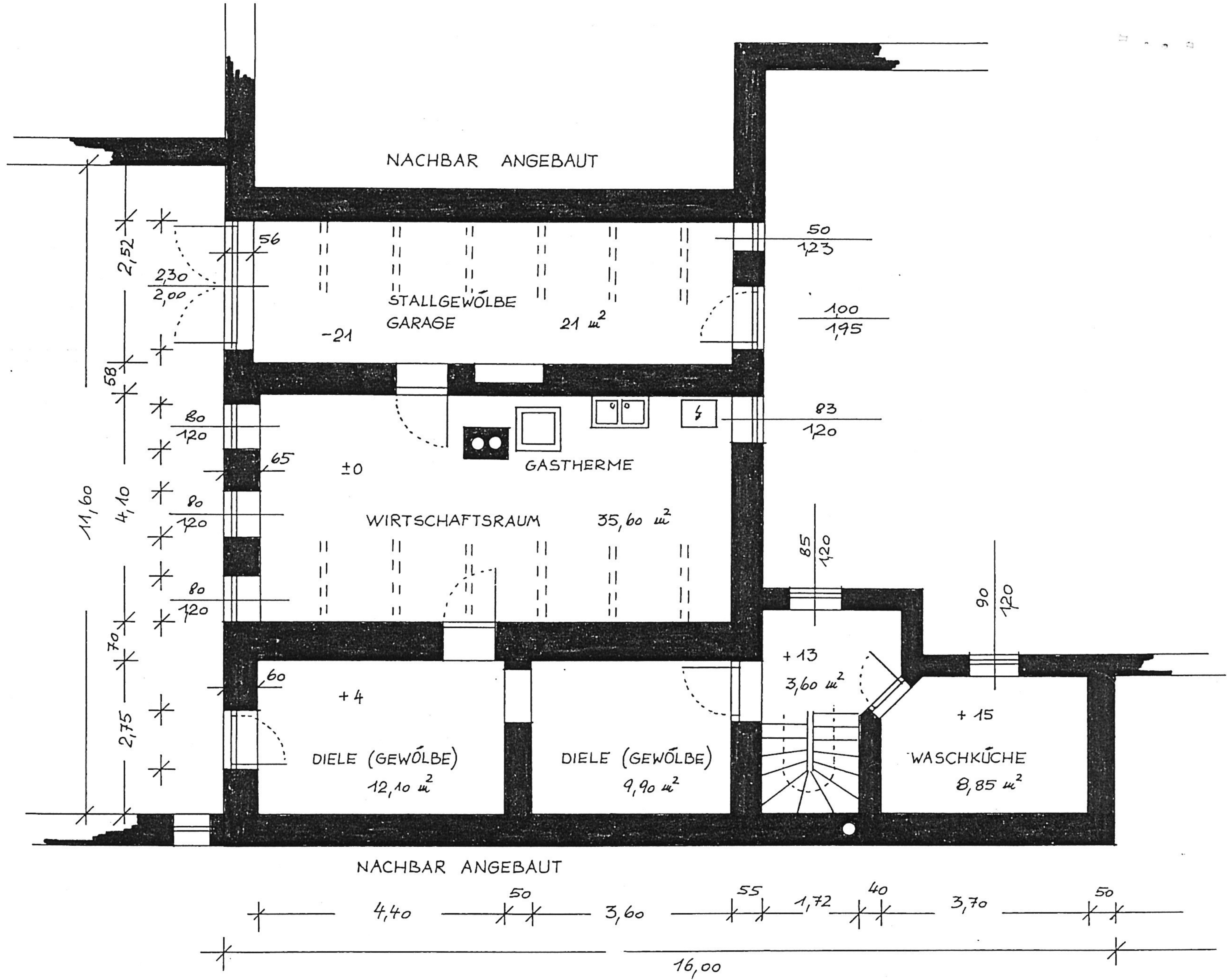
GRUNDRISS 91,05 m 2
